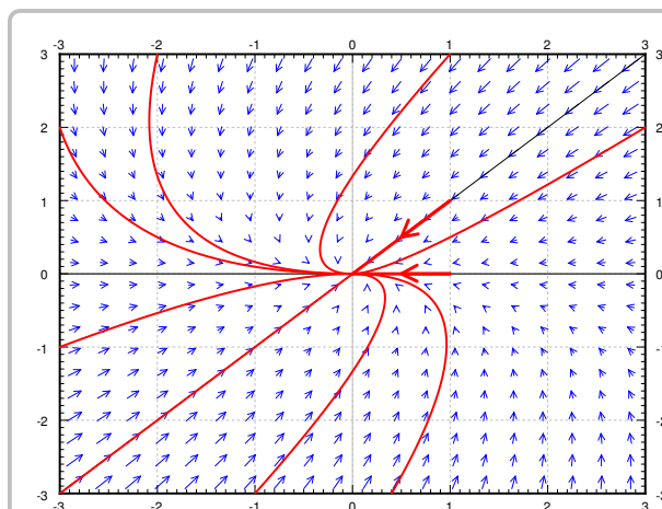
Figure 4.8: Example sink vector field with eigenvectors and solutions.
