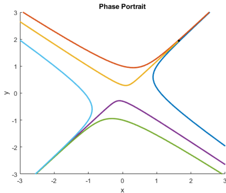
Figure A.11: Sample output from the phasePortrait244 function.
