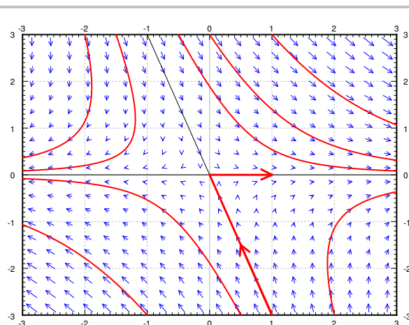
Figure 4.9: Example saddle vector field with eigenvectors and solutions.
